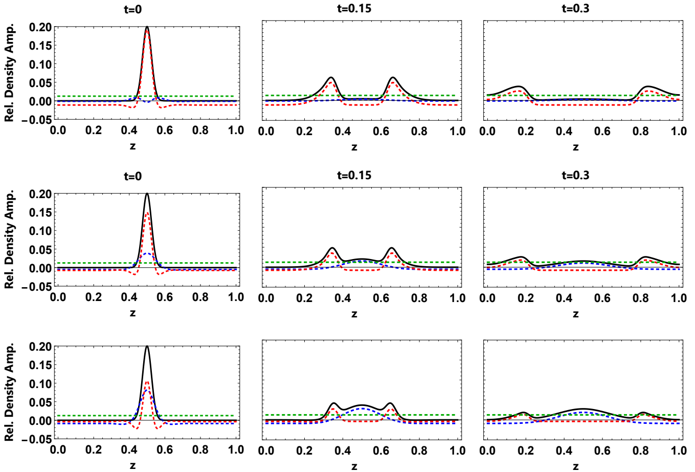
Figure 1a. Evolution of the initial Gaussian perturbation with width w = l/40 situated at z_0 = l/2 . The characteristic time is set to \tau_{\text{cond}} = 25 . The top , middle and bottom rows correspond to the ratio of magnitudes A_P/A_\rho equals 1.5, 1 and 0.5, respectively. Left , middle , and right columns indicate the solutions at t = 0 , t = 0.15 , and t = 0.3 of the computational time, respectively. The black solid line corresponds to the full solution (sum of solutions for one entropy and two slow MA modes). The red and blue dashed lines indicate the sum of two slow MA modes and one entropy mode, respectively. The green dashed line corresponds to the non-oscillating and non-propagating background.
