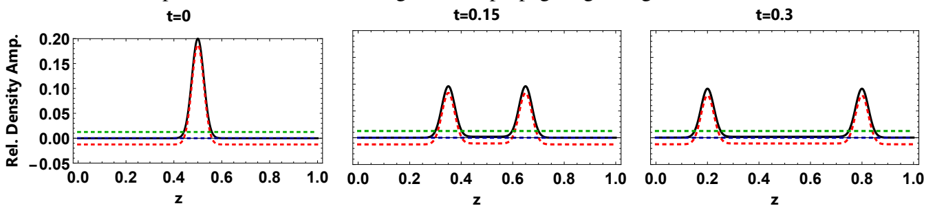
Figure 1b. Evolution of the initial Gaussian perturbation with width w = l/40 situated at z_0 = l/2 . The characteristic time is set to \tau_{\text{cond}} = 1 . Calculations are made for the ratio of magnitudes A_P/A_\rho equal to 1.
