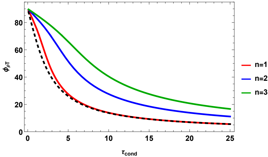
Figure 3. The phase shifts \phi_{\rho T} (23) between density and temperature perturbations as a function of dimensionless characteristic timescale \tau_{\text{cond}} (6). The red , blue , and green colors are for the first(fundamental), second, and third harmonic, respectively. The dashed line indicates the dependence described by the expression for the phase shift of fundamental harmonic obtained using assumptions of the weak impact of thermal conduction (see e.g. Owen et al. (2009)).
