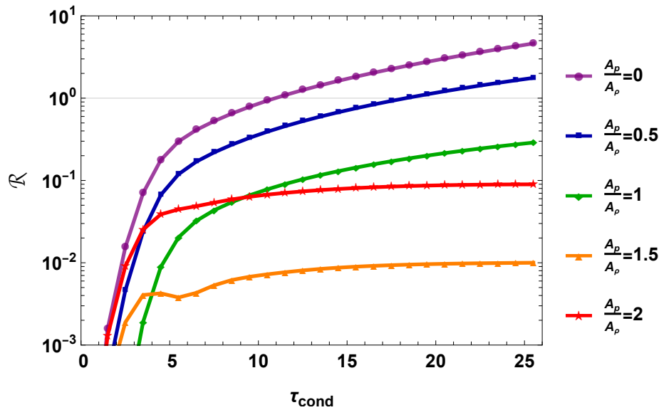
Figure 2. Dependence of the ratio \mathcal{R} (22) on dimensionless characteristic timescale \tau_{\text{cond}} (6) calculated for different values magnitude ratio A_P/A_\rho .
